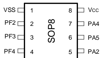
图 3-5 SOP8 Pinout1 PY32T020L1xS7-B (Top view)
