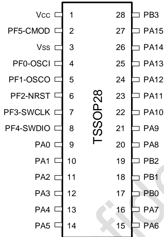
图 3-1 TSSOP28 Pinout1 PY32T020G1xP7-B (Top view)
