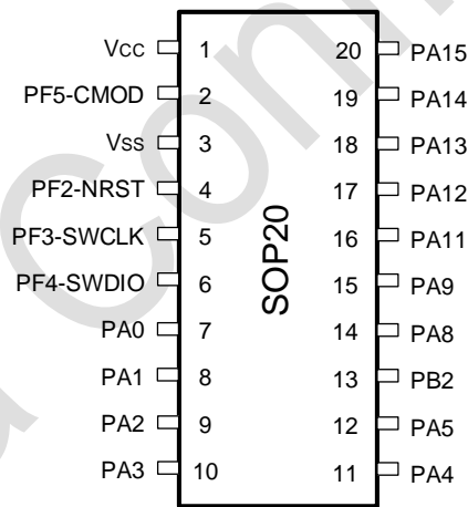
图 3-4 SOP20 Pinout1 PY32T020F1xS7-B (Top view)
