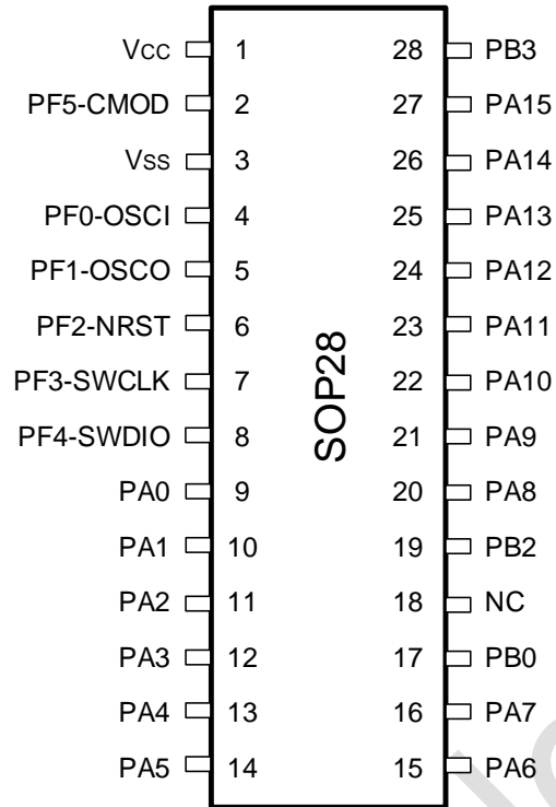
图 3-3 SOP28 Pinout4 PY32T020G4xS7-B (Top view)
